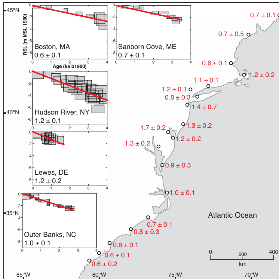
Figure 1. Rate of late Holocene relative sea-level rise with 2 \sigma errors for 19 locations along U.S. Atlantic coast. Inset plots are examples of locations with sea-level index points plotted as calibrated age before A.D. 1900 versus change in relative sea level (RSL) relative to mean sea level (MSL) in A.D. 1900 (m). Red line is linear regression for each site. Rates and errors shown to 1 decimal place. MA—Massachusetts; ME—Maine; NY—New York; DE—Delaware; NC—North Carolina.
