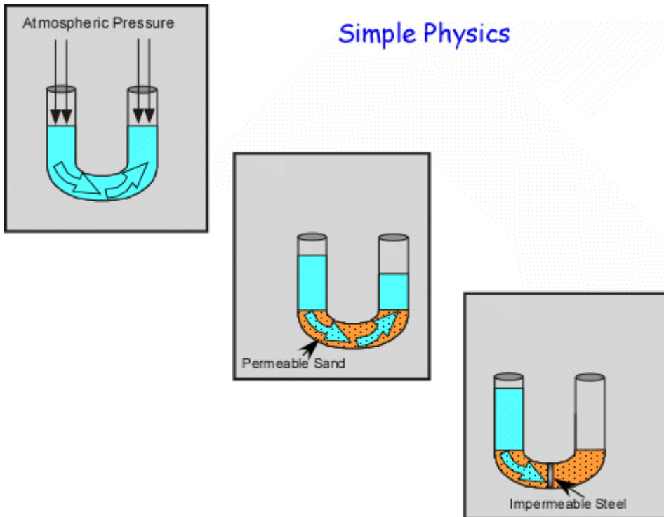
Figure 20. A simple thought experiment illustrates the principle of hydrostatic pressure by imagining a U-shaped glass tube. The water levels in each side of the tube rise to the same level because both sides of the tube are subject to the same pressure (atmospheric pressure). If a permeable material like sand is placed in the bottom of the tube and water is poured into one side, the water will find its way through the intricate pathways between the sand grains and will eventually, although not instantaneously rise to the same level on the other side of the tube. If an impermeable barrier is placed in the sand in the bottom of the tube, then the water will not get from one side to the other.
